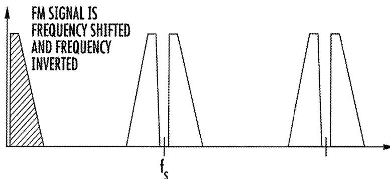
FREQUENCY SPECTRUM AFTER UNDERSAMPLING AT HALF THE ORIGINAL SAMPLING RATE
