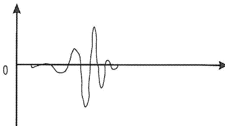
Wavelet function \Psi(t)
