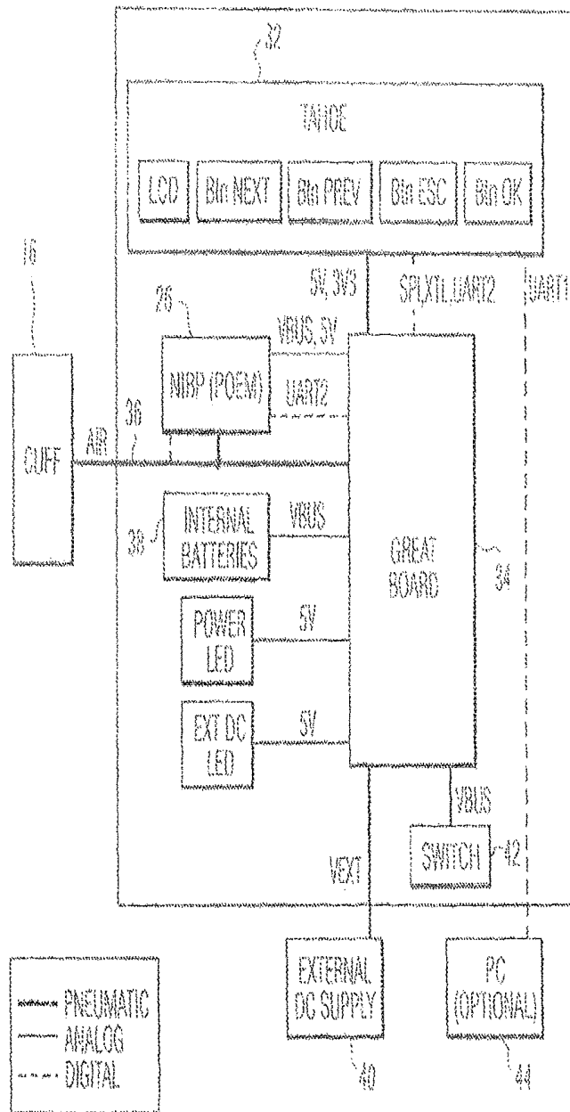
Fig 1: Device Block Diagram
