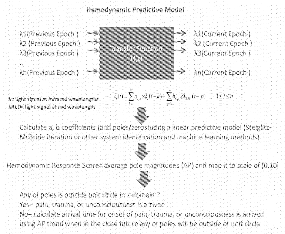
Figure A7: Pipeline to predict hemodynamic changes using a predictive model.
