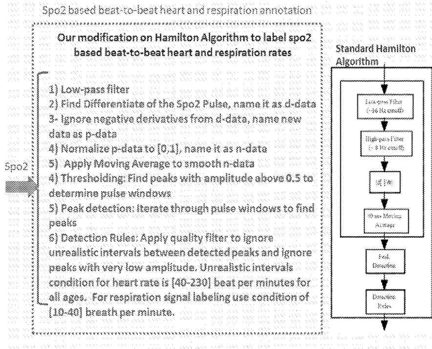
Figure A6. Spo2 based beat-to-beat heart and respiration annotation.
