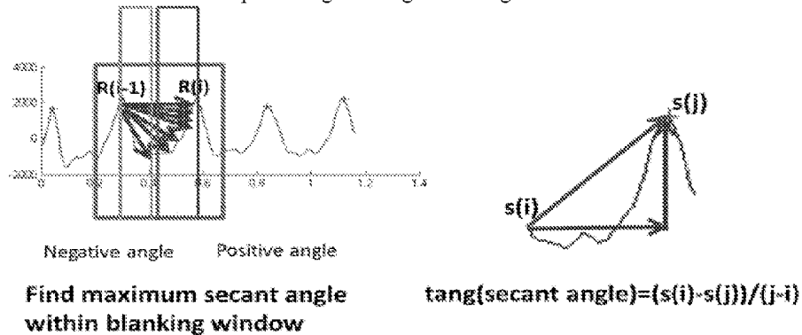
Figure A5. Detection of envelope of signal using secant angle. For Upper envelope detector searches for maximum secant angle within a user defined blanking window. For lower envelope it searches for minimum secant angle within the blanking window.
