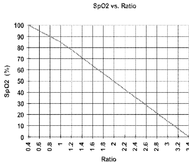
Figure A3: Ratio is used as the input to a “lookup table”. The SpO2 value is the result of the “lookup” function
