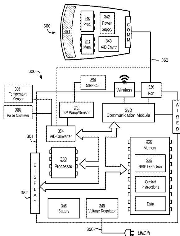
COMPONENTS OF VITAL SIGNS MONITOR
