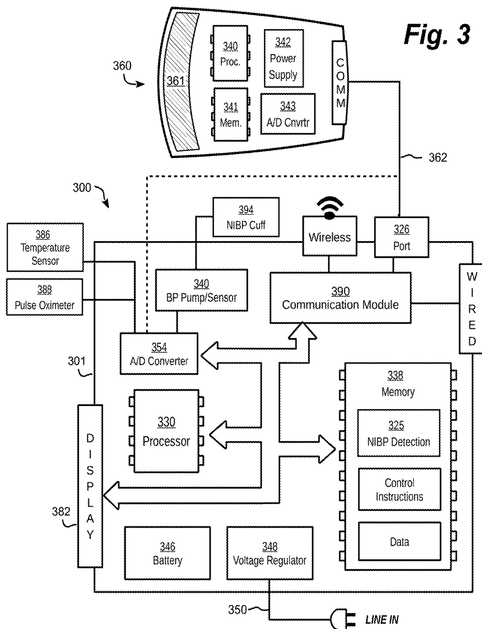
COMPONENTS OF VITAL SIGNS MONITOR
