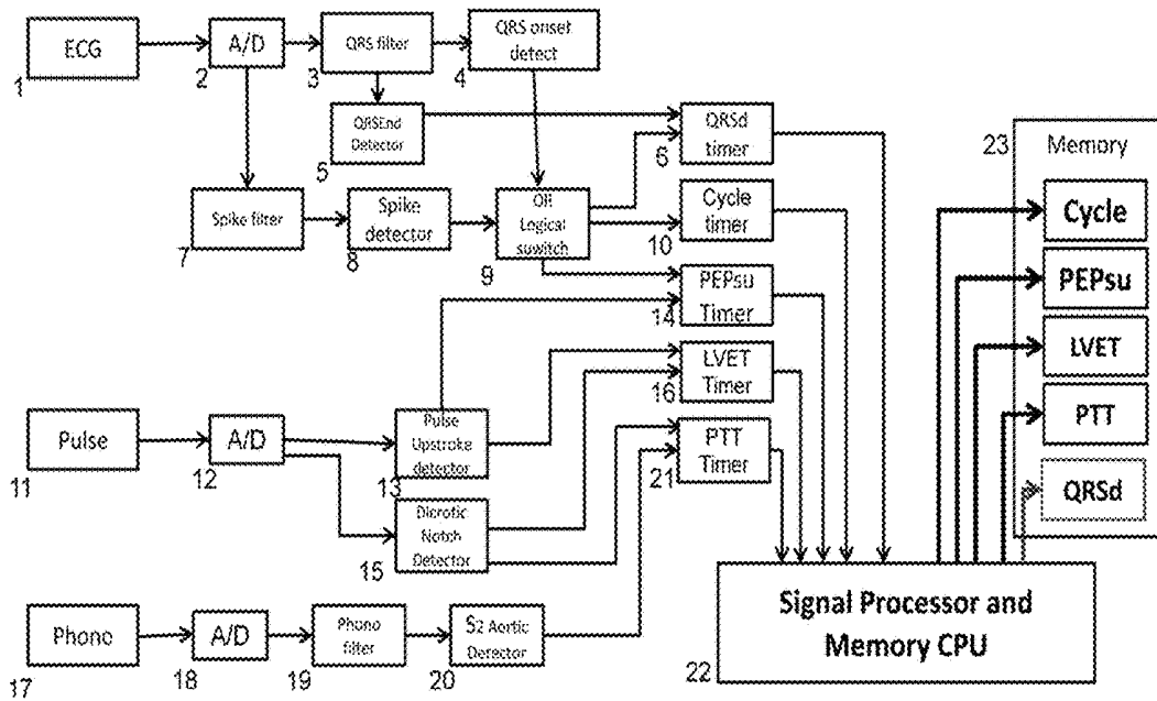
Figure 3. Flow chart of electronic circuitry
