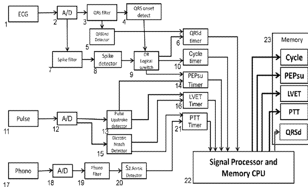
Flow chart of electronic circuitry
