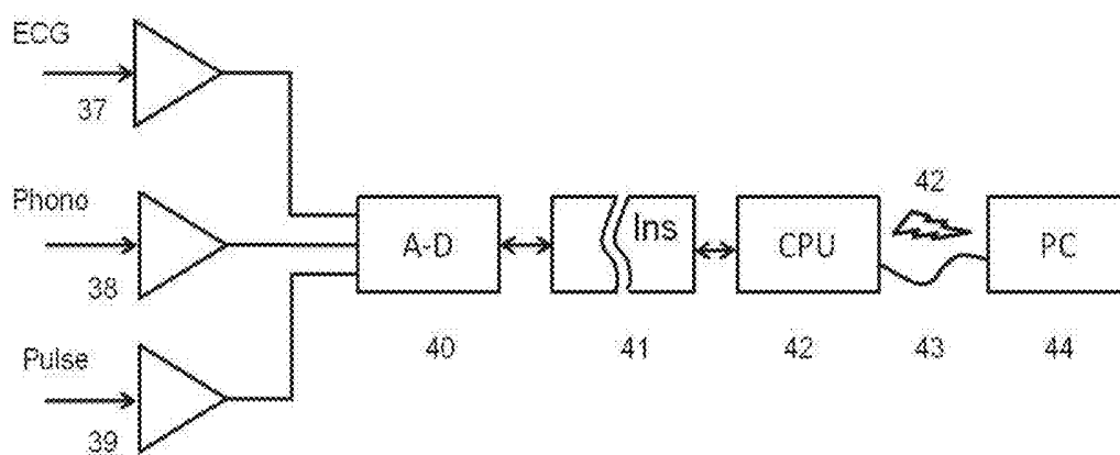
Figure 6. Alternative embodiment of the invention.
