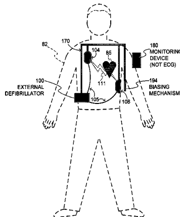
WEARABLE DEFIBRILLATOR SYSTEM
