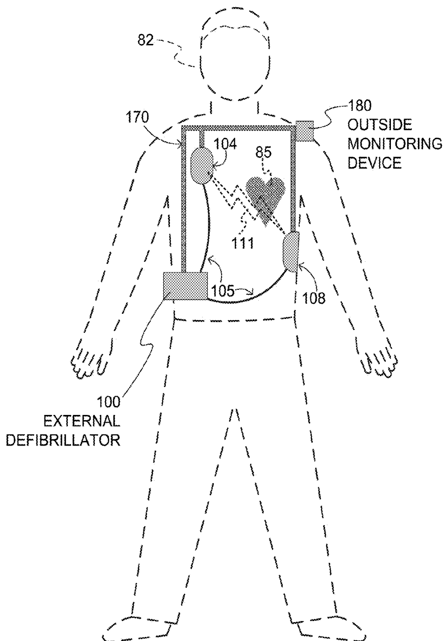
WEARABLE CARDIAC DEFIBRILLATOR (WCD) SYSTEM WITH COMPONENT
