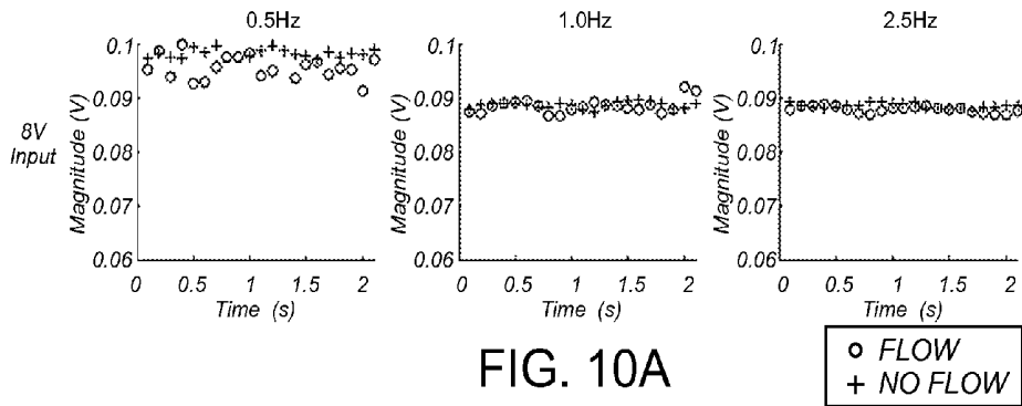
Elongate Member #1 Resistive Member #4: Magnitude Plot
