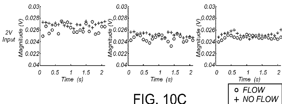
Elongate Member #1 Resistive Member #4: Magnitude Plot
