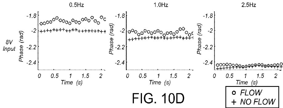
Elongate Member #1 Resistive Member #4: Phase Plot
