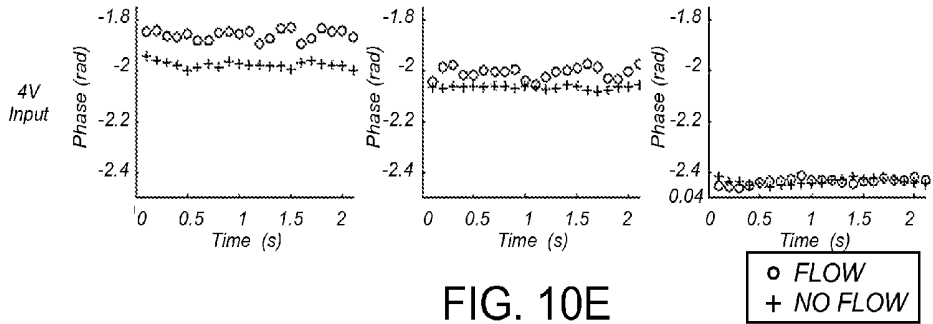
Elongate Member #1 Resistive Member #4: Phase Plot
