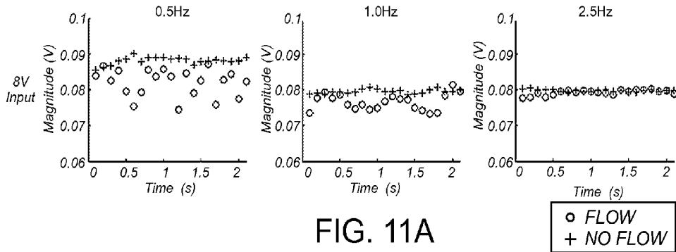
Elongate Member #2 Resistive Member #3: Magnitude Plot
