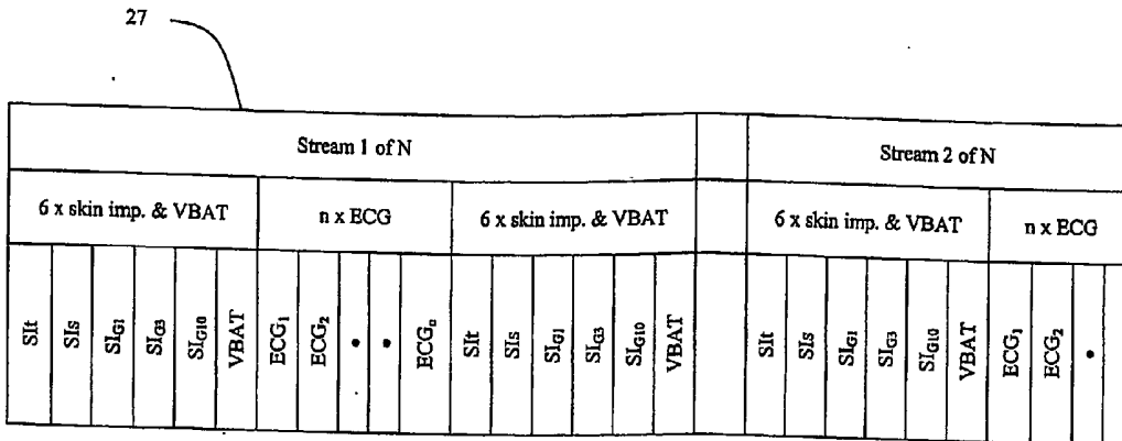
Figure 5c: Transmitter data sequence stream
