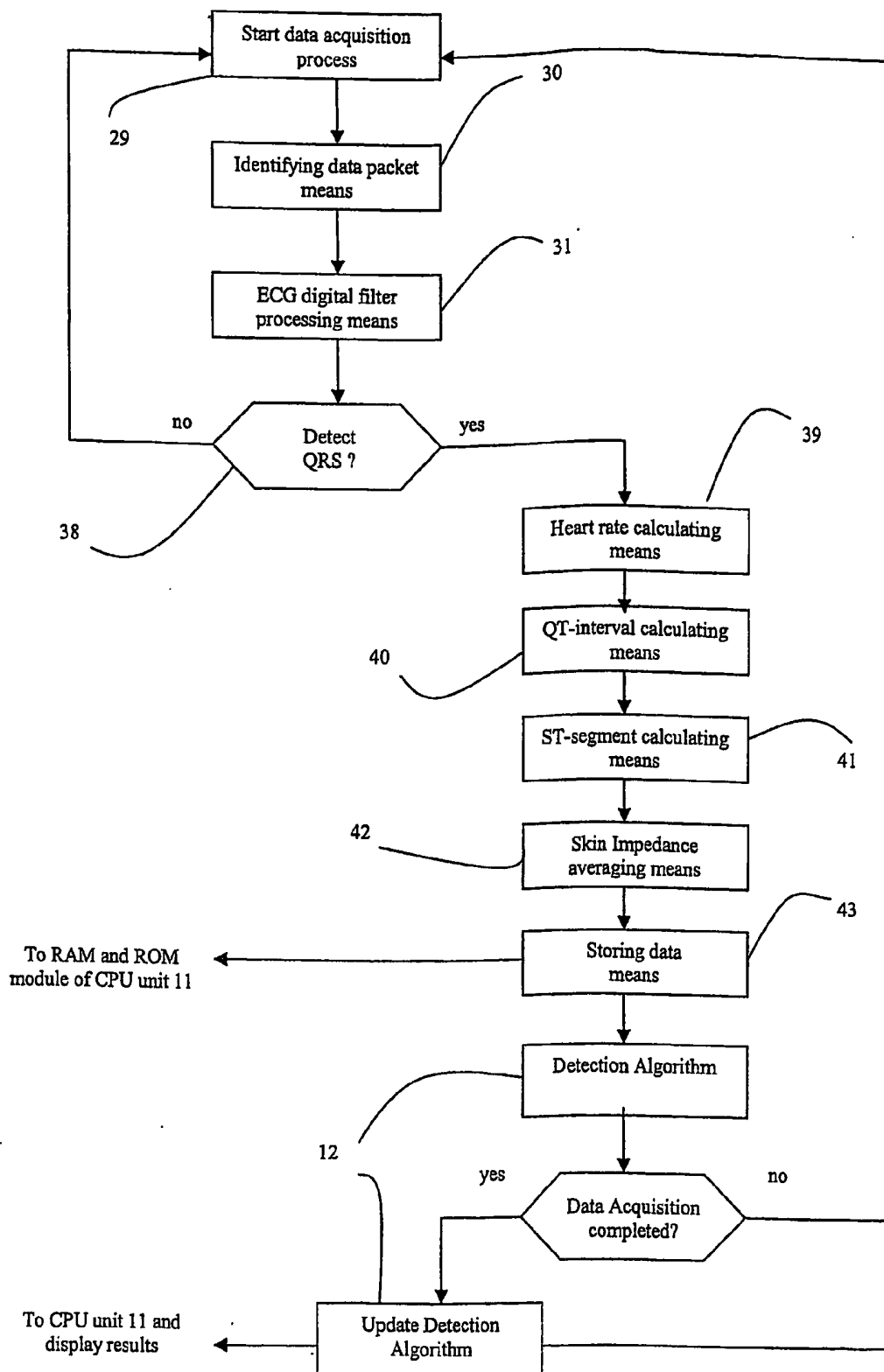
Figure 6a: Data acquisition process
