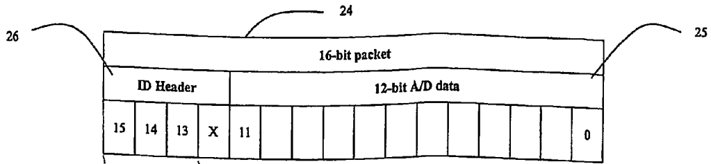
Figure 5a: Transmission Data Format
