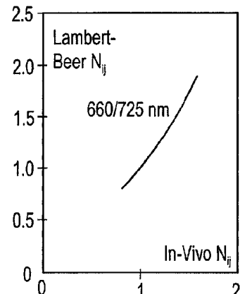
FIG. 4c PRIOR ART
