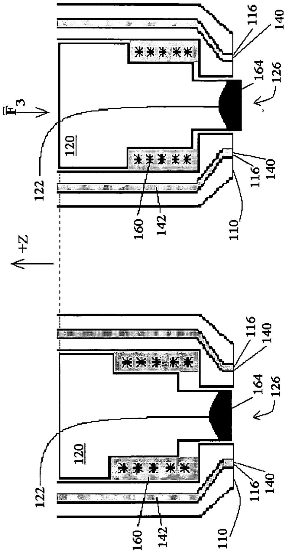
Piston Deployed Figure 8D
