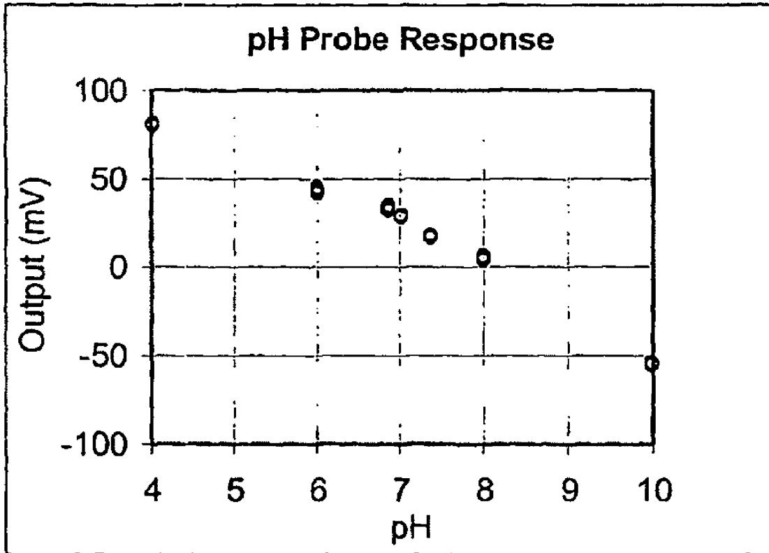
Chart 6: pH sensor performance
