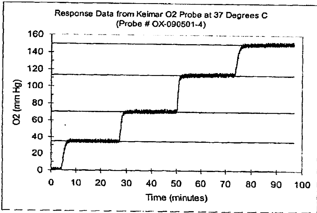
Chart 2: Oxygen sensor response
