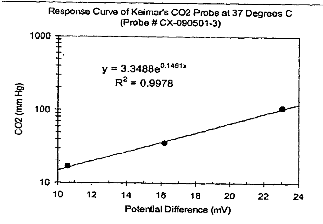
Chart 4: Carbon dioxide sensor performance
