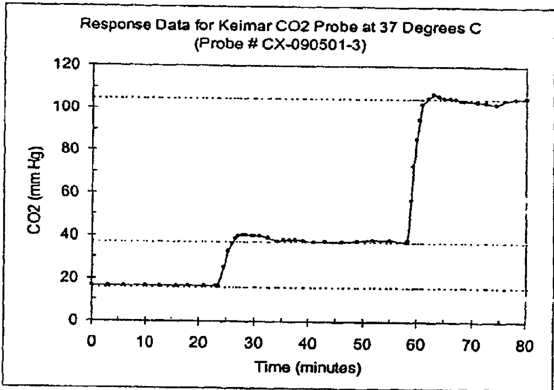
Chart 5: Carbon dioxide sensor response
