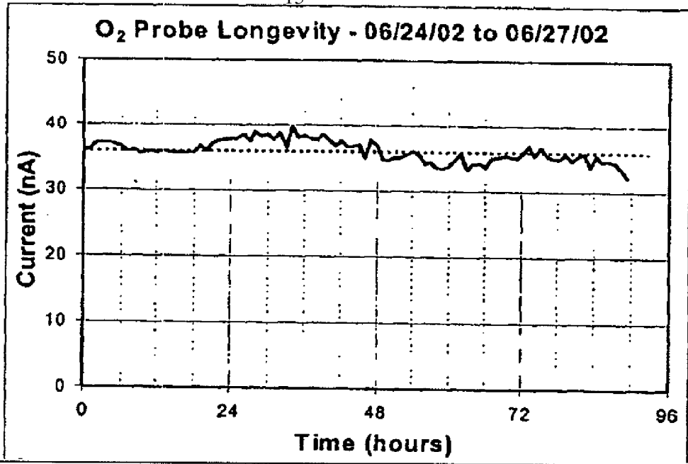
Chart 3: Oxygen sensor longevity
