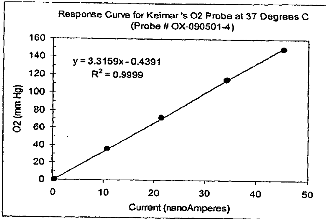
Chart 1: Oxygen sensor performance
