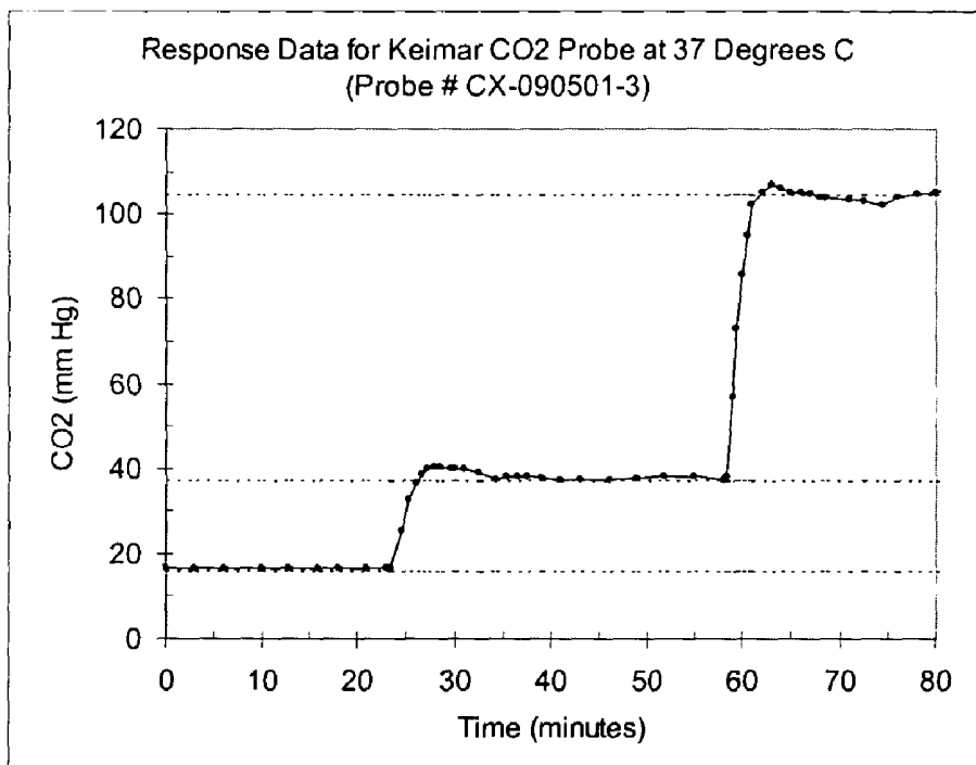
Chart 5: Carbon dioxide sensor response
