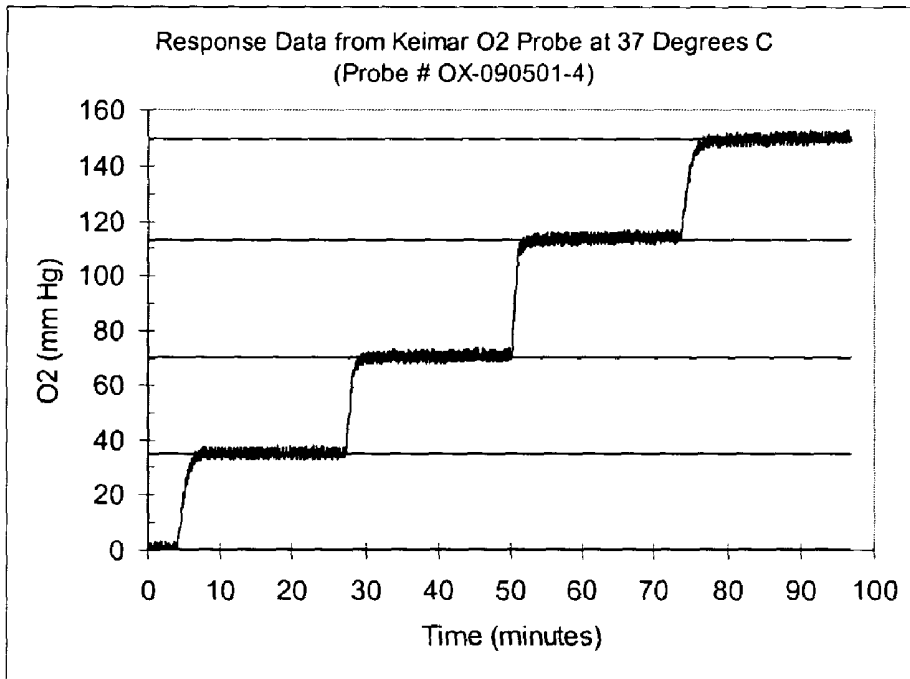
Chart 2: Oxygen sensor response
