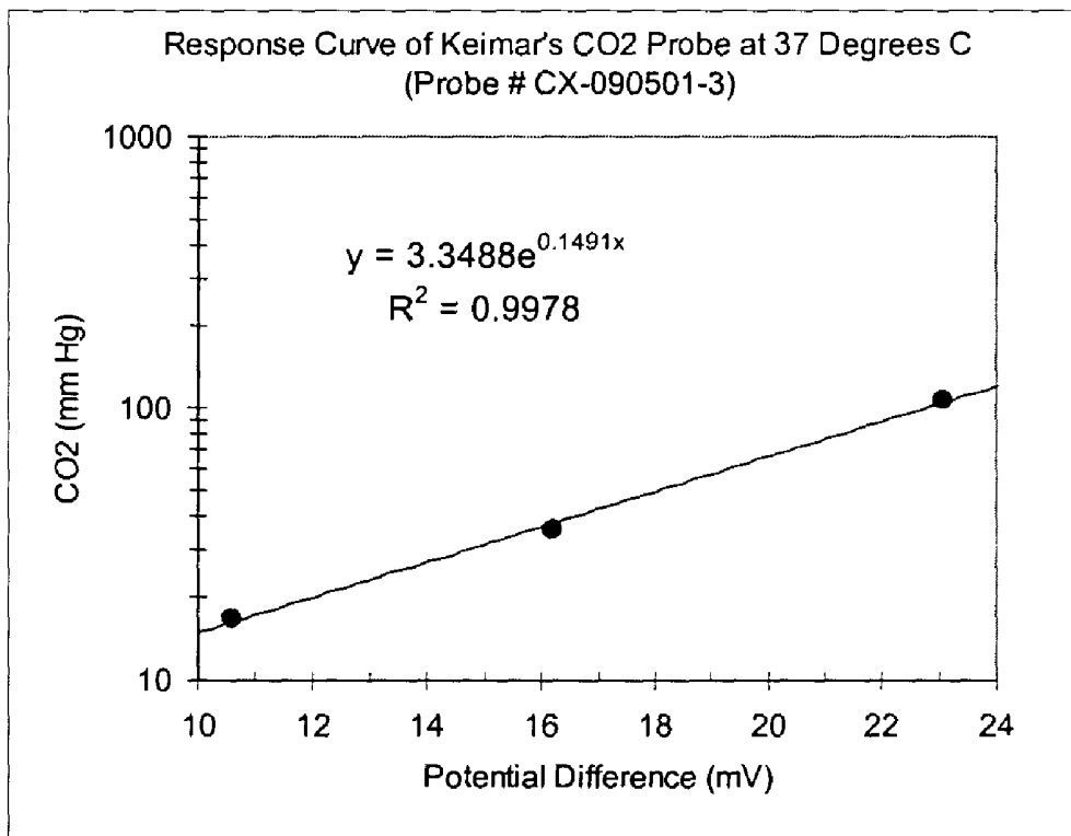
Chart 4: Carbon dioxide sensor performance
