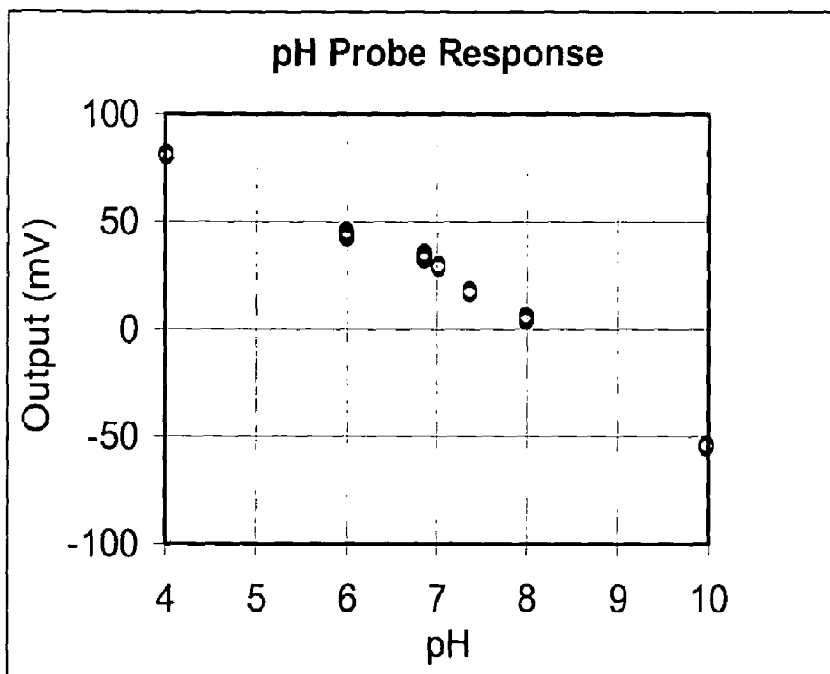
Chart 6: pH sensor performance
