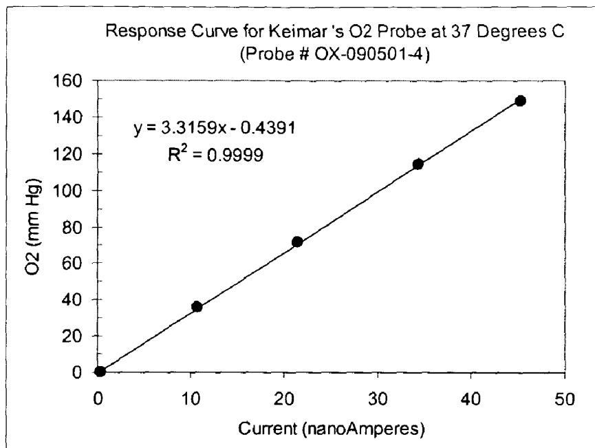
Chart 1: Oxygen sensor performance
