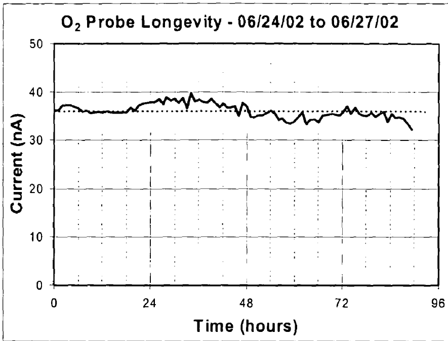
Chart 3: Oxygen sensor longevity
