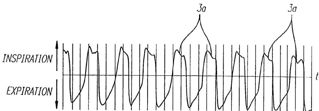
FIG. 3 AIRFLOW TO AND FROM CPAP GENERATOR
