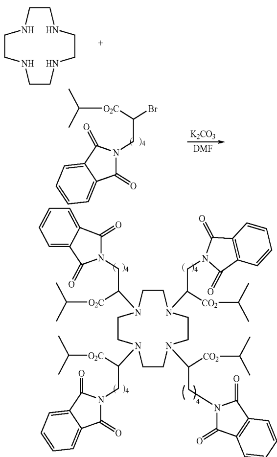
C. Tetraisopropyl 1,4,7,10-tetraazacyclododecane-1,4,7,10-tetra[2-6-(N-phtalimido)-hexanoate
