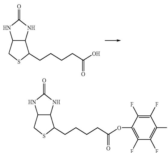
A. Biotin Tetrafluorophenyl Ester
