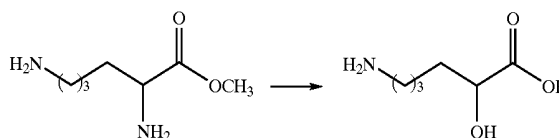
A. (-)-6-Amino-2-hydroxyhexanoic Acid [ Chem. Pharm. Bull. 1976, 24, 621]
