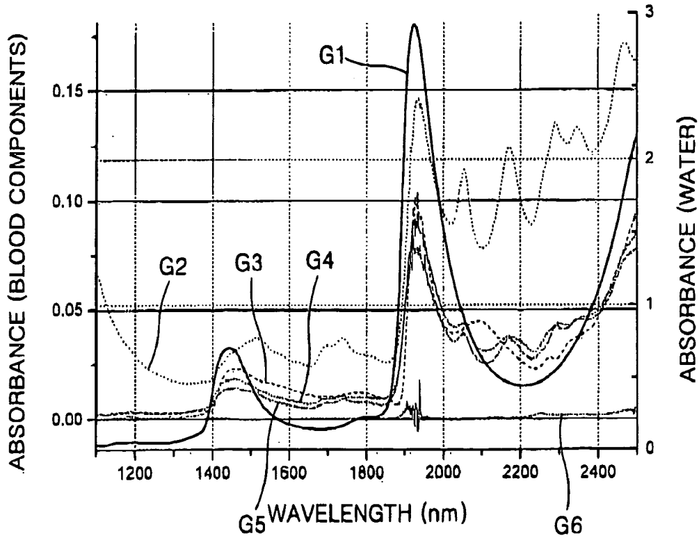
FIG. 2 (PRIOR ART)
