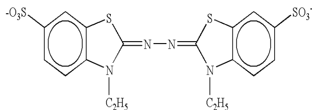
Substrate/oxidized form of ABTS
