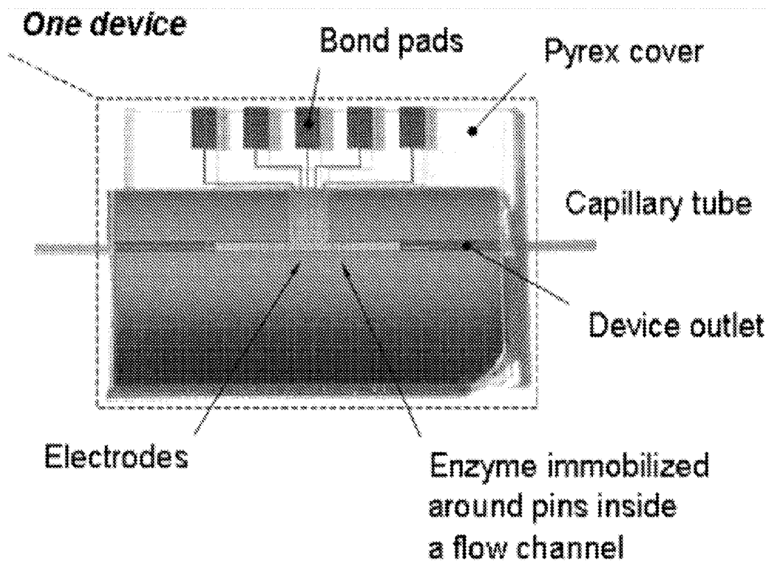
Photo of a glucose sensor integrated in a flow channel.
