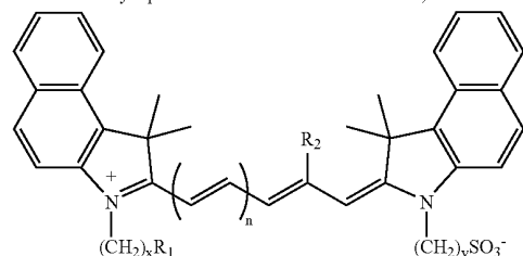
General Cyanine Dye
