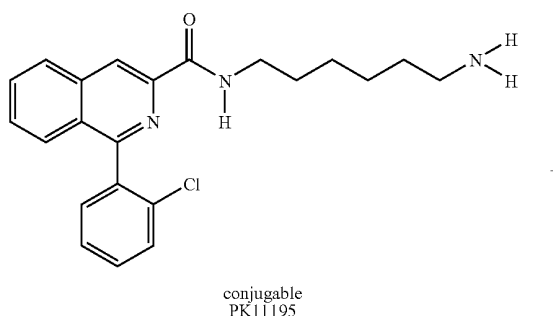
Scheme 1— Conjugation of Succinimidyl Dye to conjugable PK11195
