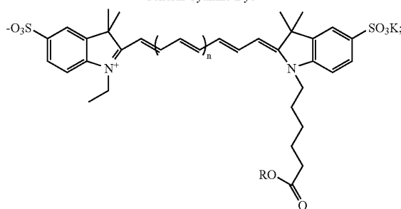
CY-Family of dyes
