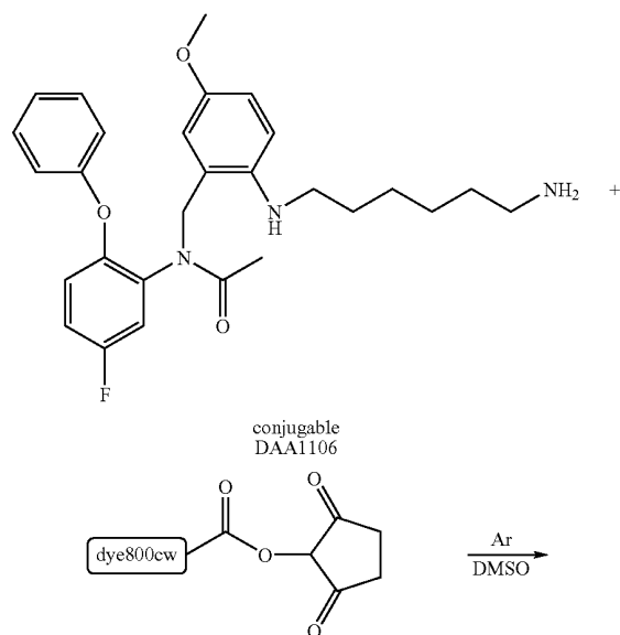
Scheme 5. Reaction scheme for dye800CW-DAA1106
