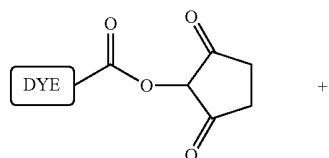
Scheme 2— Conjugation of Succinimidyl Dye to glucosamine
