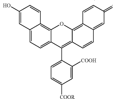
Carboxynaphthofluorescein abs/em = 580 nm, 690 nm
