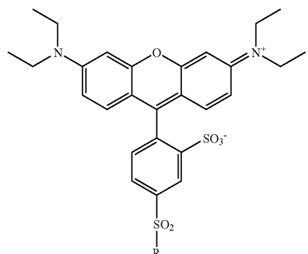
Lissamine-Rhodamine abs/em = 560 nm, 590 nm
