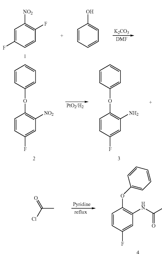
Scheme 4— Synthesis of conjugatable DAA1106
