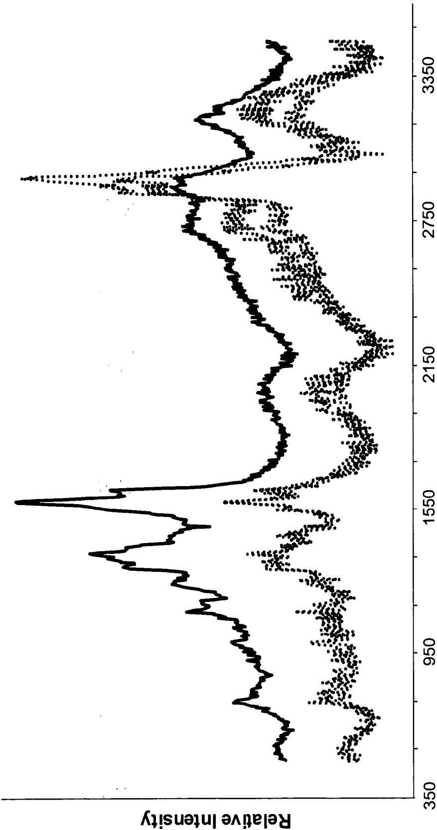
Wavenumber (cm -1 )
