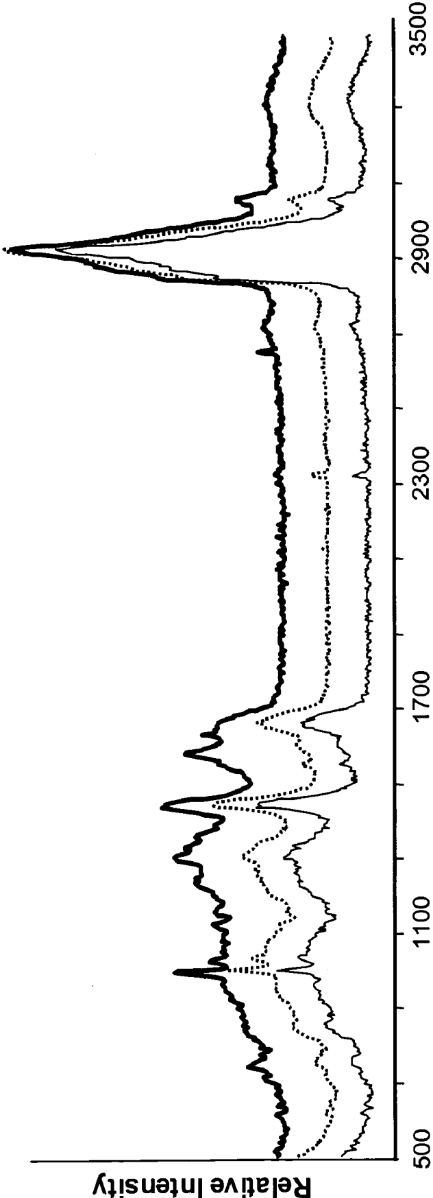
Wavenumber (cm -1 )
