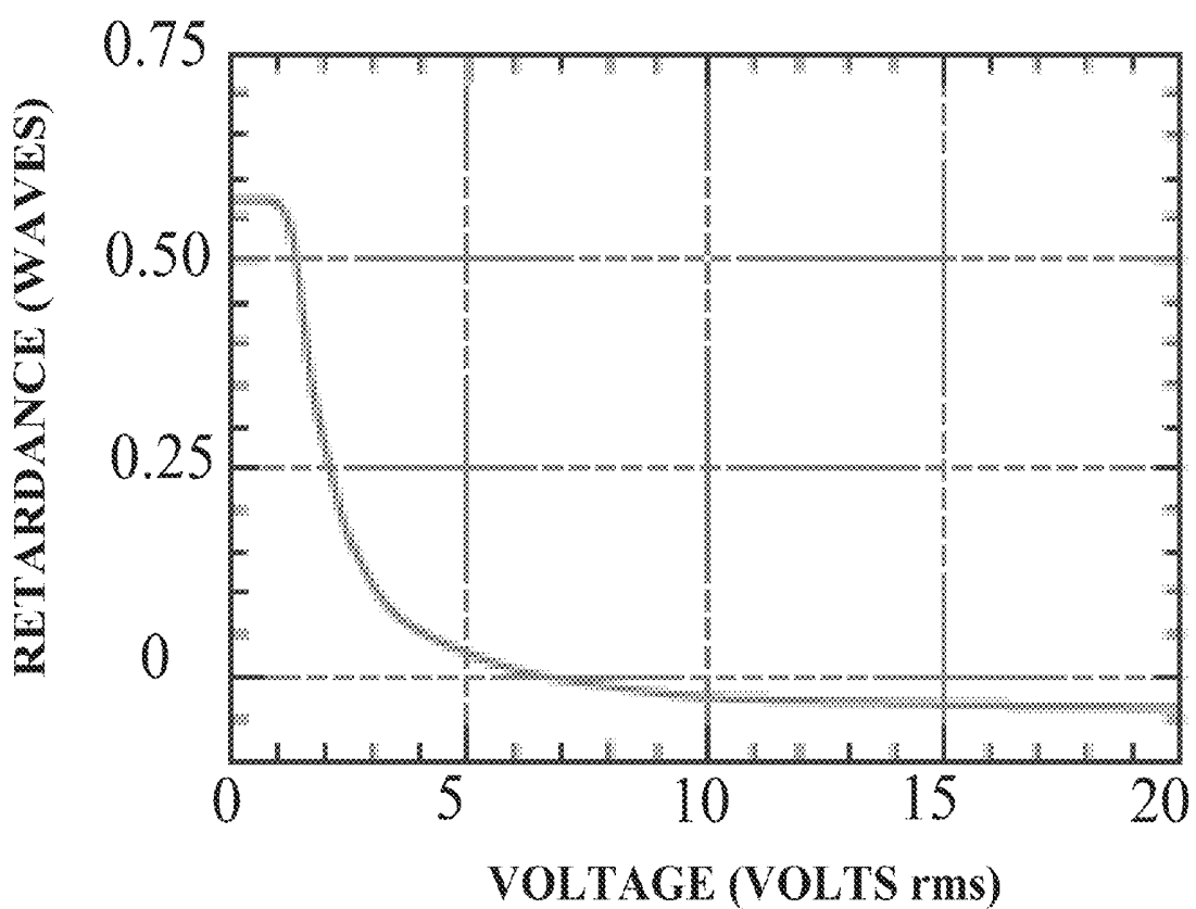
Retarder Tuning curve
