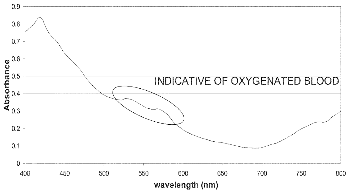
Plot of spectral absorbance of middle finger (no rubber band) using image cube with horizontal polarization showing effect of oxygenated blood
