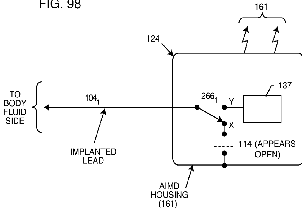
MRI GRADIENT (LOW) FREQUENCY MODEL
