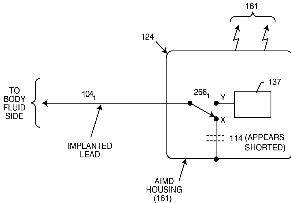
MRI PULSED RF (HIGH) FREQUENCY MODEL
