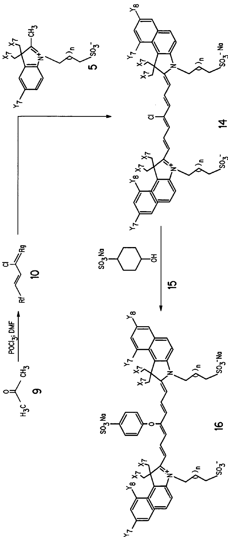
FIG. 4 : n = 1-3 ; X_7 = H , OH ; Y_7 = H , SO_3^- , CO_2H , CH_2CO_2H , CH_2OH ; R_f = (CH_3)_2N^+ or CHO
