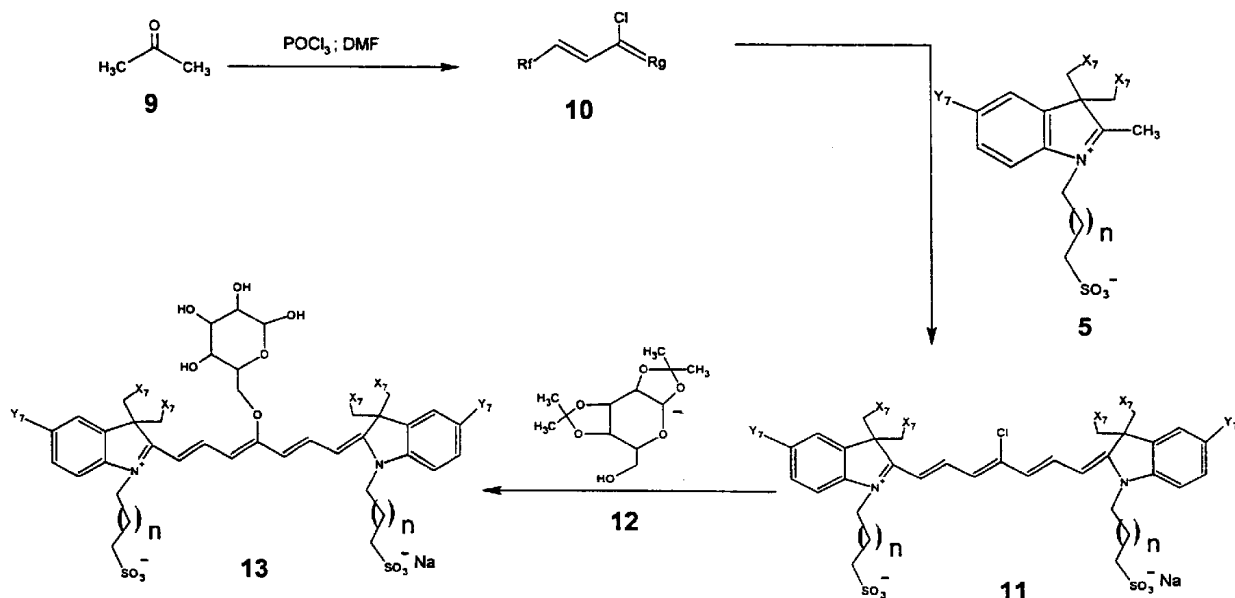
Figure 3: n = 1-3 ; X_7 = \text{H, OH} ; Y_7 = \text{H, SO}_3^-, \text{CO}_2\text{H, CH}_2\text{CO}_2\text{H, CH}_2\text{OH} ; R_f = (\text{CH}_3)_2\text{N} or \text{OH} ; R_g = (\text{CH}_3)_2\text{N}^+ or \text{CHO}
