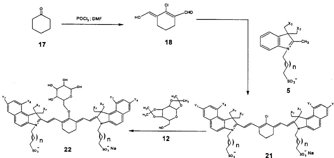
Figure 6: n = 1-3; X 7 = H, OH; Y 7 , Y 8 = H, SO 3 - , CO 2 H, CH 2 CO 2 H, CH 2 OH
