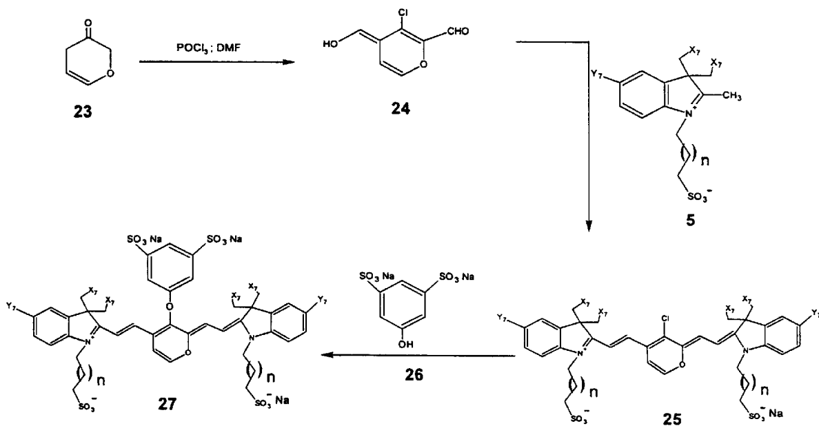
Figure 7: n = 1-3 ; X_7 = \text{H}, \text{OH} ; Y_7, Y_8 = \text{H}, \text{SO}_3^-, \text{CO}_2\text{H}, \text{CH}_2\text{CO}_2\text{H}, \text{CH}_2\text{OH}
