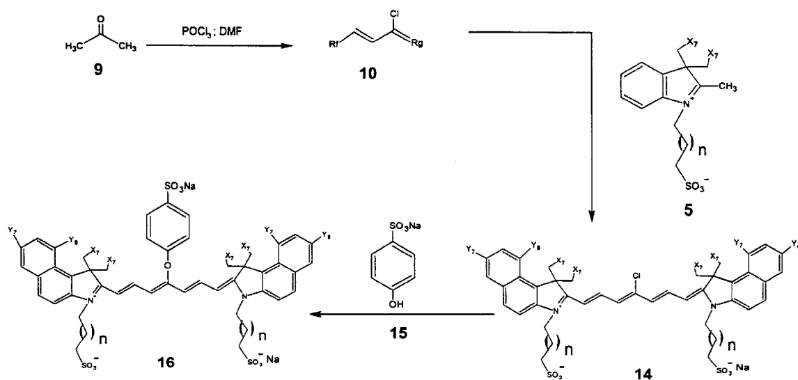
Figure 4: n = 1-3 ; X_7 = \text{H, OH} ; Y_7 = \text{H, SO}_3^-, \text{CO}_2\text{H, CH}_2\text{CO}_2\text{H, CH}_2\text{OH} ; R_f = (\text{CH}_3)_2\text{N} or \text{OH} ; R_g = (\text{CH}_3)_2\text{N}^+ or \text{CHO}
