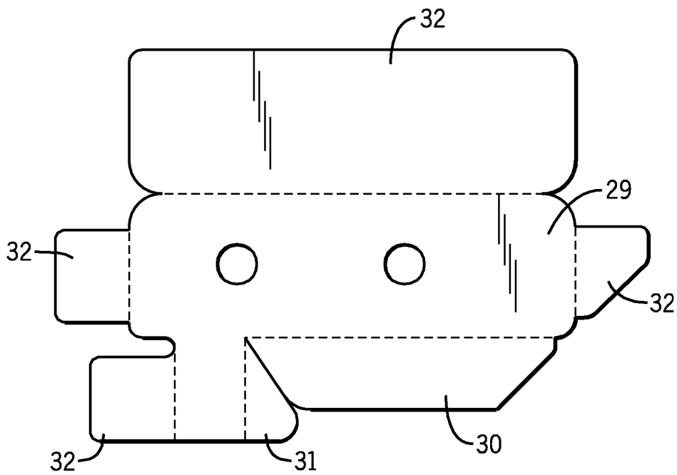
FIG. 3 PRIOR ART
