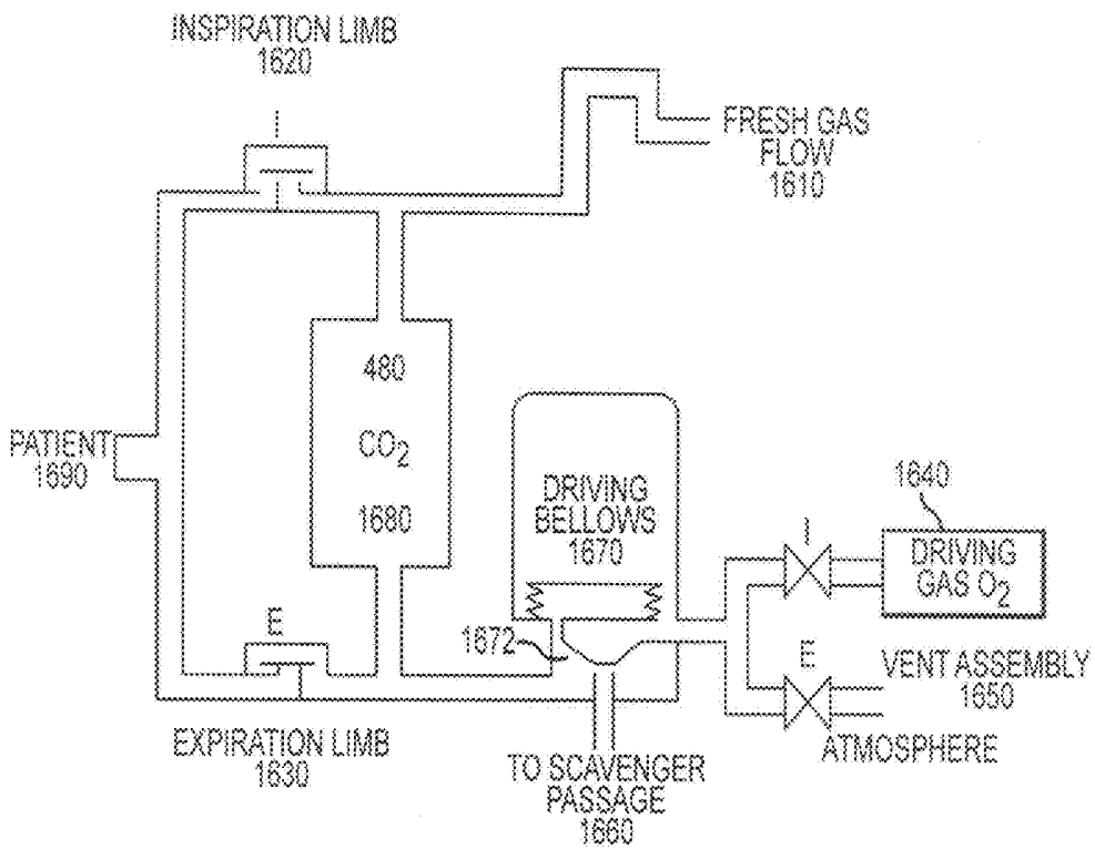
ANESTHESIA MACHINE
