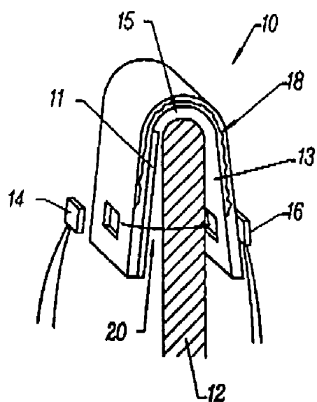
FIG. 1 PRIOR ART
