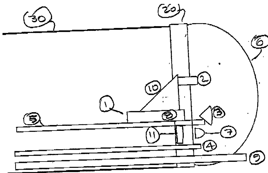
Figure 2A: Optical Head Schematic—Side View
