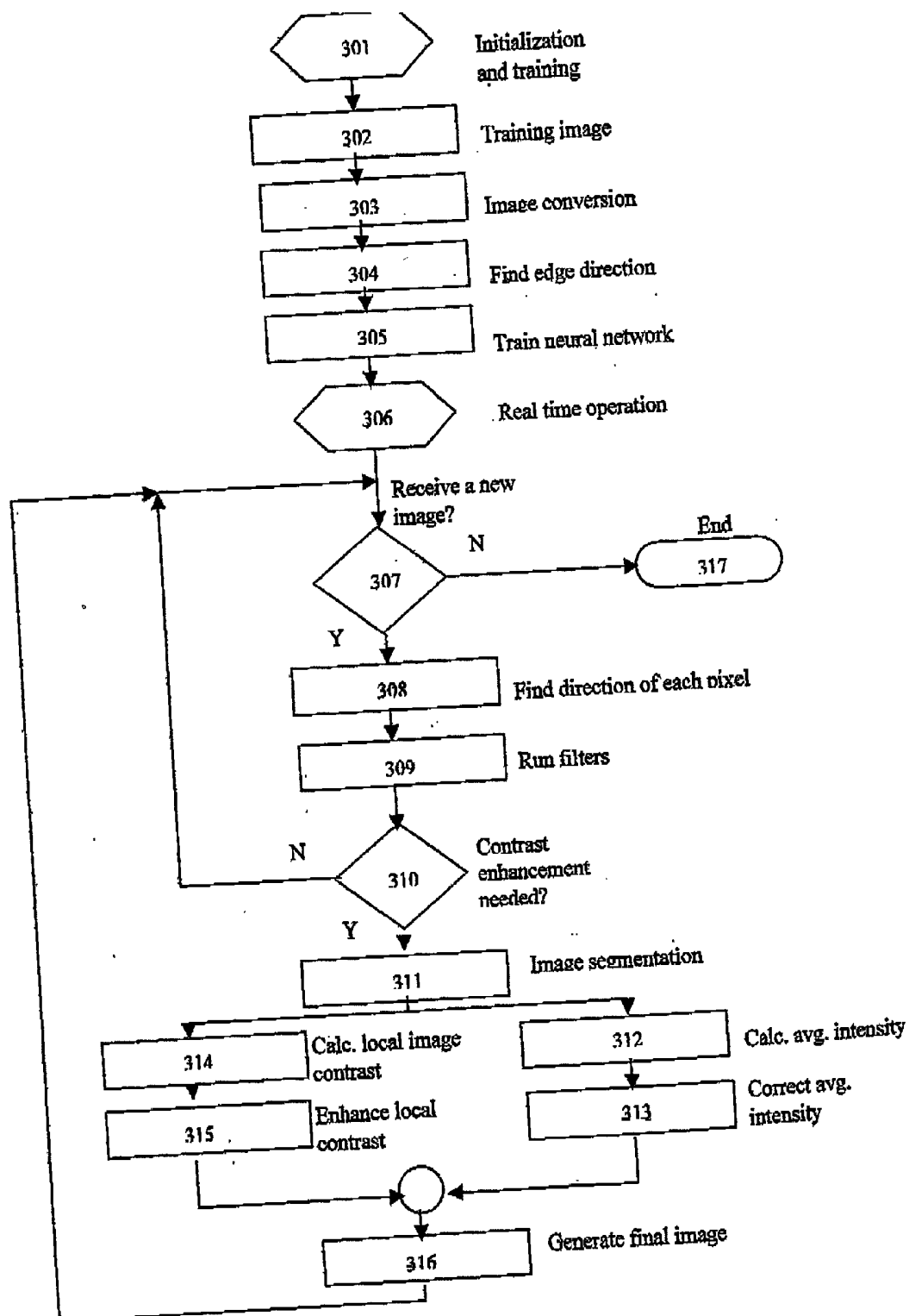
Figure 7: Block diagram of post-processing algorithm
