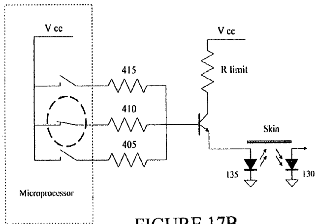
FIGURE 17B
