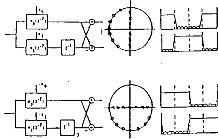
FIGURE 9. HILBERT TRANSFORM ALL-PASS FILTER REALIZATION AS TRANSFORMED HALF BAND FILTER
