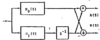
FIGURE 8. COMPLEMENTARY LOWPASS AND HIGHPASS FILTERS FROM 2-PATH ALL-PASS NETWORK
