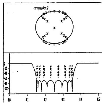
FIGURE 11. SPECTRUM OF ITERATED 2-PATH FILTER: POLYNOMIALS IN Z^4
