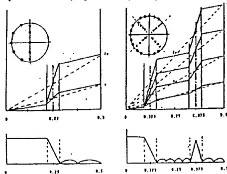
FIGURE 6. TYPICAL PHASE RESPONSES OF ALL-PASS FILTER PATHS, AND CORRESPONDING MAGNITUDE RESPONSES.
