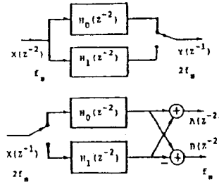
FIGURE 10. RESAMPLING 2-PATH ALL-PASS FILTER
