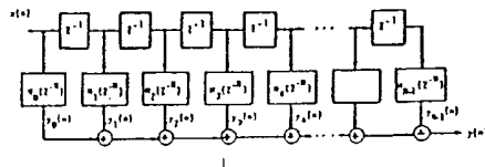
FIGURE 4A. ALL-PASS FILTER STRUCTURE
