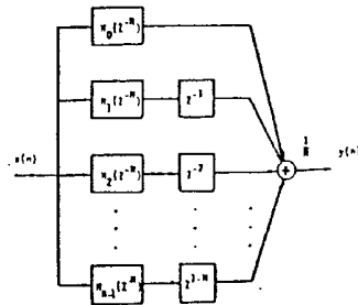
FIGURE 4B. POLYPHASE ALL-PASS STRUCTURE
