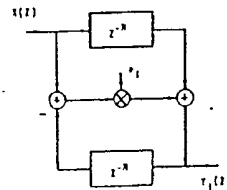
FIGURE 3. M-TH ORDER ALL-PASS SUBFILTER
