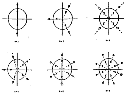
FIGURE 5. POLE-ZERO DISTRIBUTION FOR M-TH ORDER ALL-PASS SUBFILTERS
