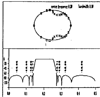
FIGURE 14. BANDPASS TRANSFORMATION OF ALL-PASS FILTER
