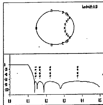
FIGURE 13. LOWPASS TRANSFORMATION OF ALL-PASS FILTER
