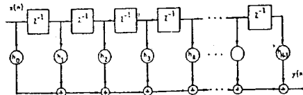
FIGURE 1. TAPPED DELAY LINE FIR FILTER
