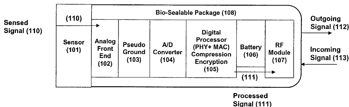
Medical Monitoring Device (100)
