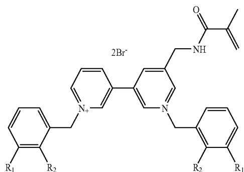
3,3'-oBBV; R_1 = H , R_2 = B(OH)_2 3,3'-mBBV; R_1 = B(OH)_2 , R_2 = H
