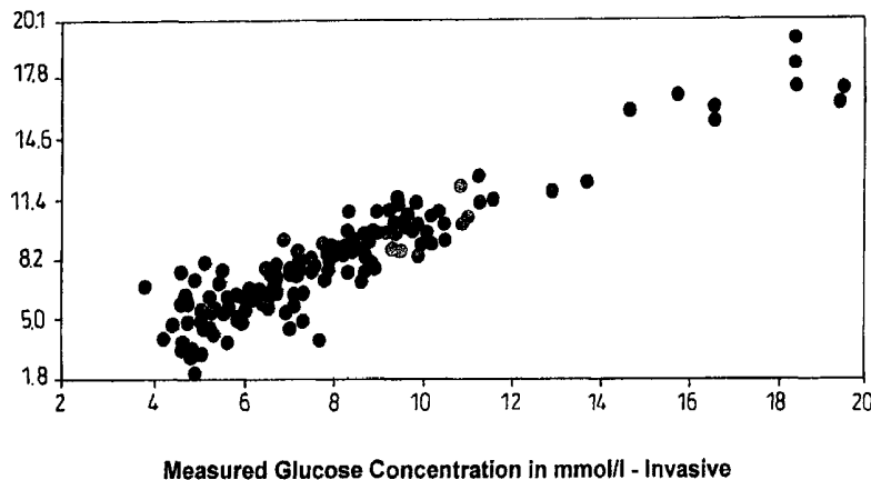
Non-invasive versus Invasive Blood Glucose Measurements
