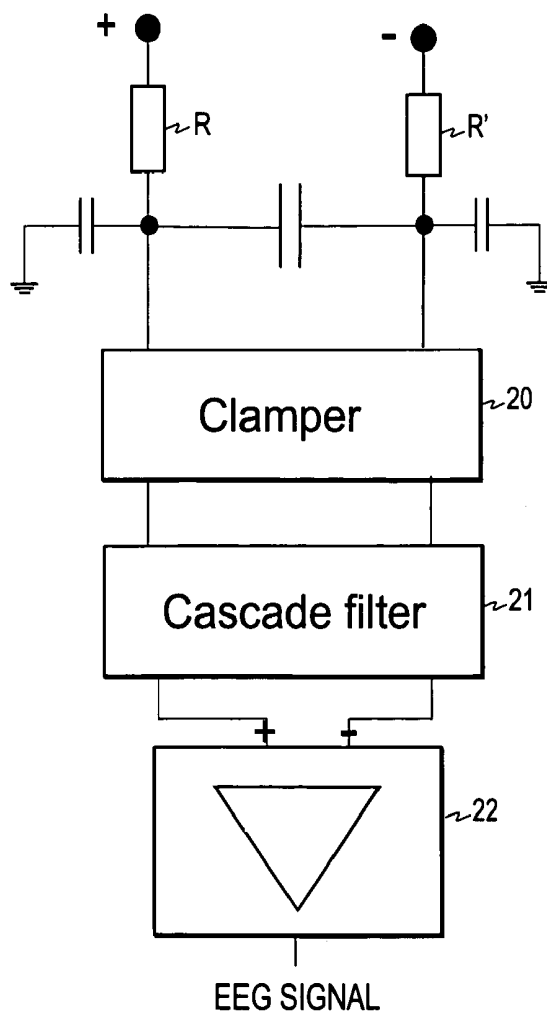
FIG. 3 Prior art
