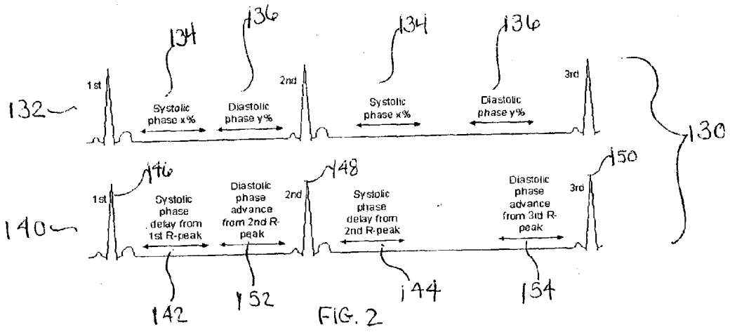
PRIOR ART
