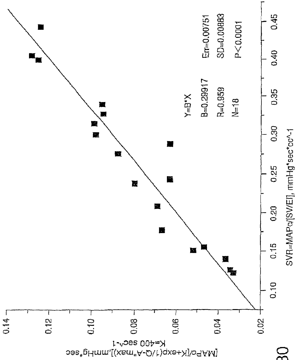
FIG. 1, SV/Rc IN TERMS OF MAPc AND Q-A n max
