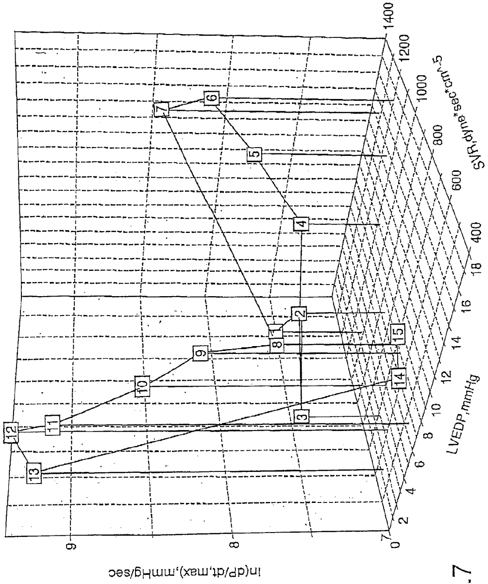
FIG. 2, INVASIVE HEMODYNAMIC VECTOR SPACE, H'
