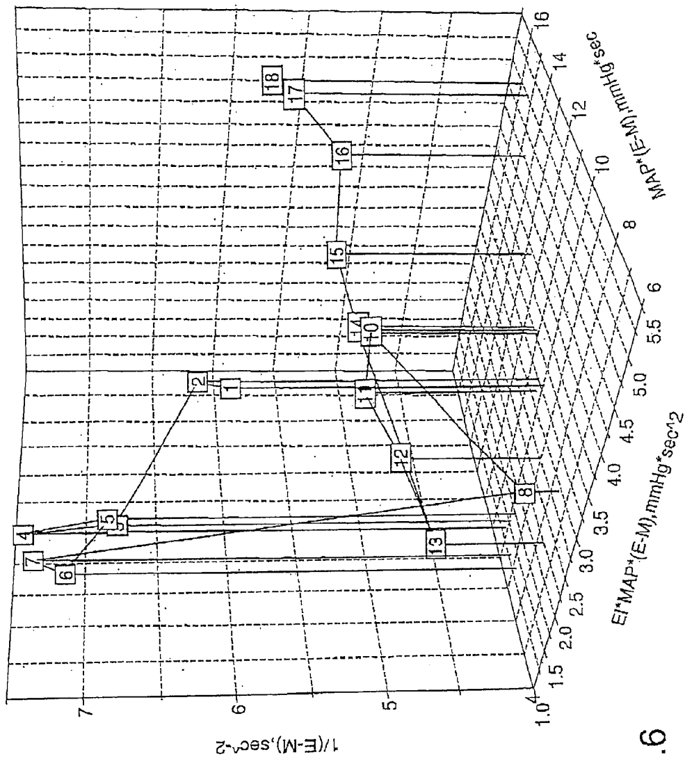
FIG 1, NONINVASIVE HEMODYNAMIC VECTOR SPACE, N
