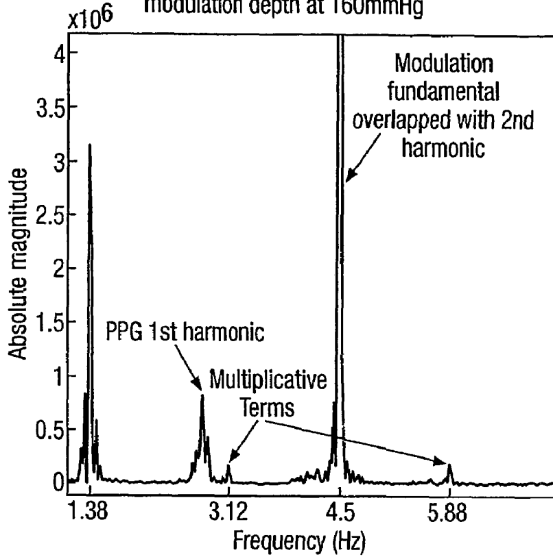
Fig.7c. Modulation frequency at 5Hz and modulation depth at 160mmHg
