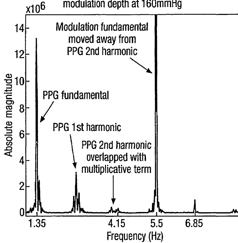
Fig.7e. Optimised modulation frequency in this particular embodiment
