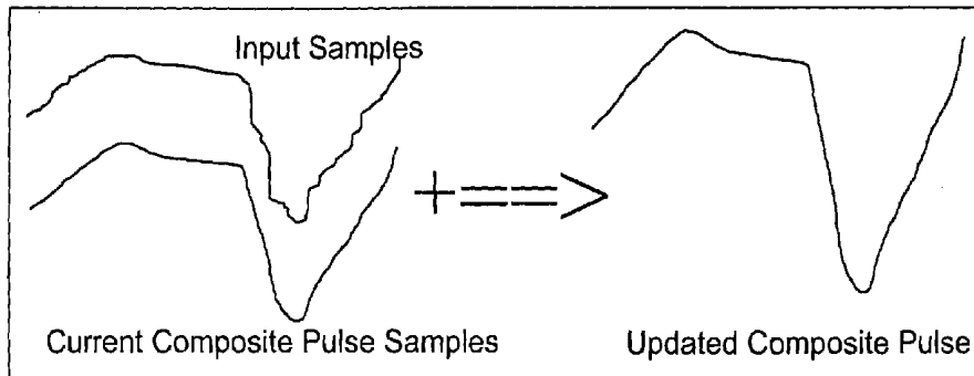
FIG. 3 Composite Pulses are updated by averaging input samples with the existing Composite Pulse samples
