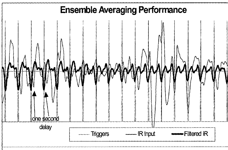
FIG. 4 Example of the Ensemble Averaging subsystem's variable weighting
