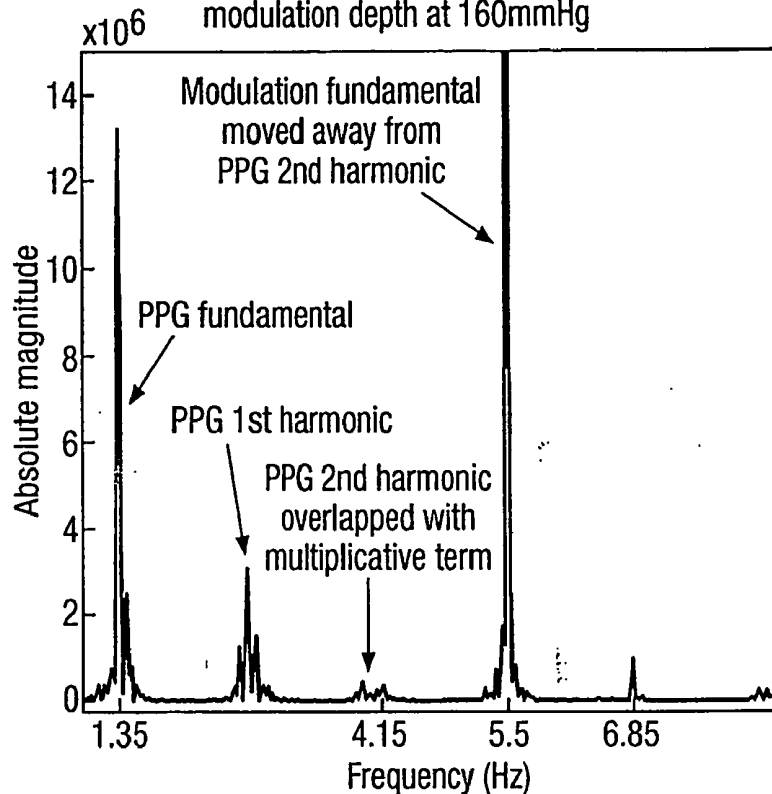
Fig.7d. Modulation frequency at 5.5Hz and modulation depth at 160mmHg
