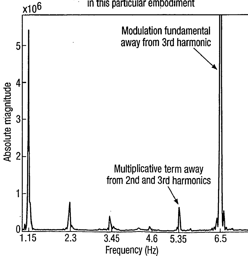
Fig.7e. Optimised modulation frequency in this particular embodiment
