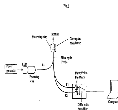
Fig1. Schematics of the fiber-optic linked pressure sensing system (FOLPS)
