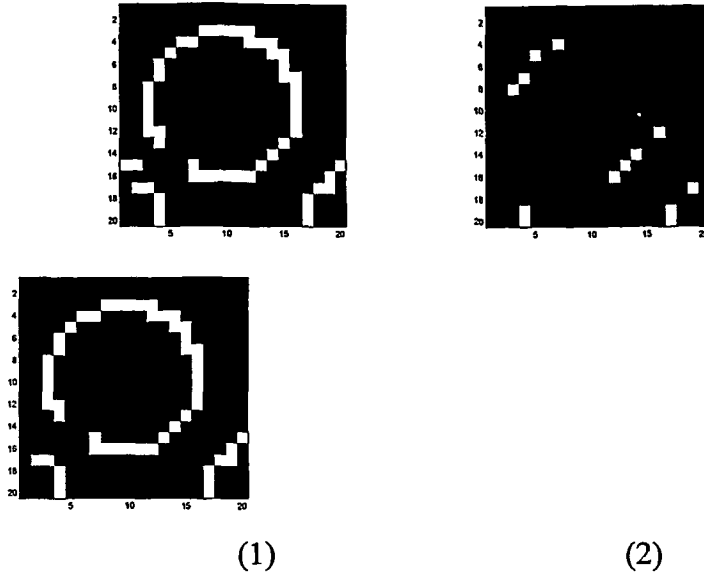
Figure L: (1) Gradient image thresholded at 3.5 – all pixels greater than 3.5 are shown as white (2) gradient image thresholded at 7, (3) Output of hysteresis threshold.
