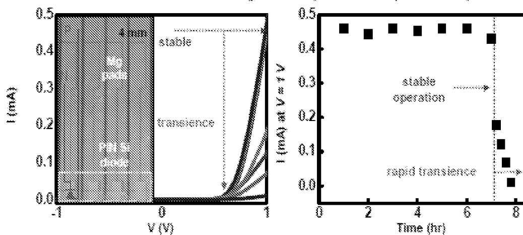
Diode on Mo foil with MgO encapsulation ( \sim 800 nm)
