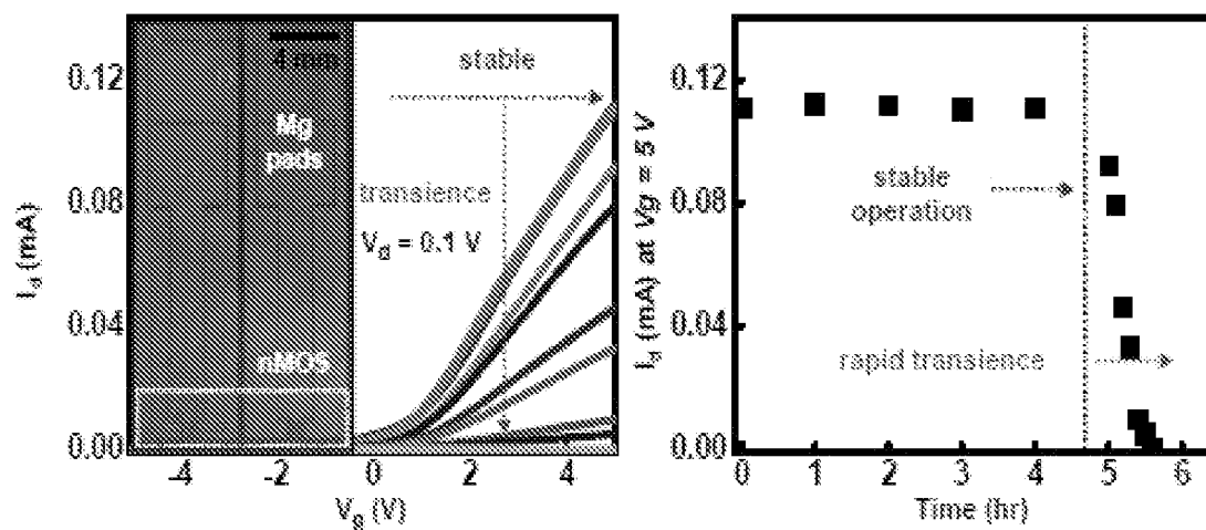
Transistor on Mo foil with MgO encapsulation ( \sim 800 nm)
