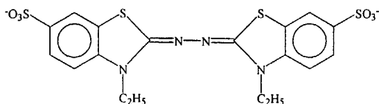
Substrate / oxidized form of ABTS
