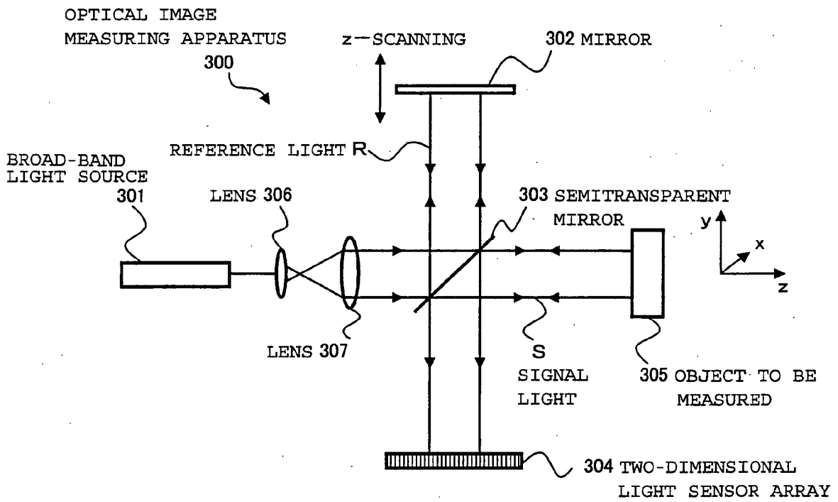
FIG. 10 PRIOR ART
