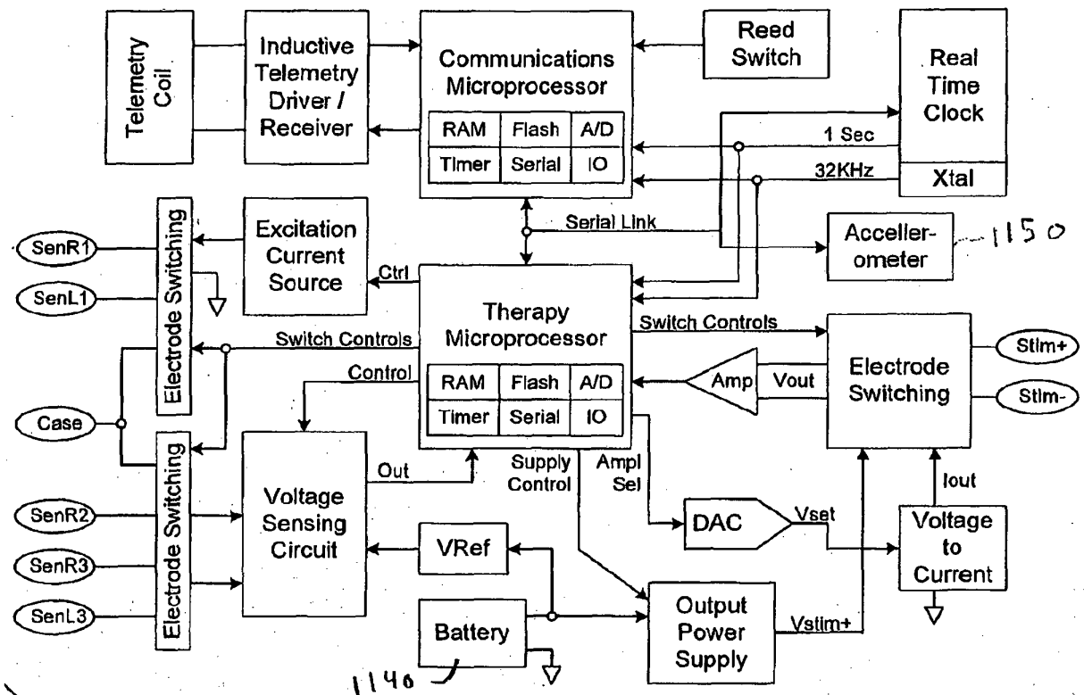
INS. (LT) FIG. 5B
