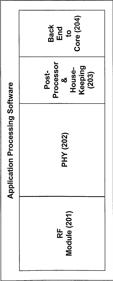
Figure 2 Base Station (200)
