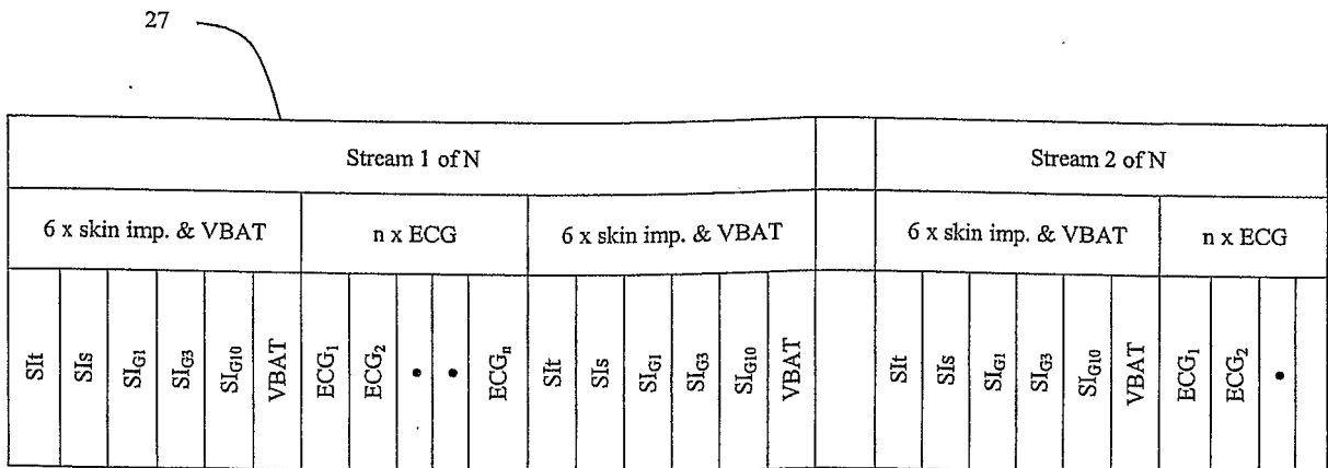
Figure 5c: Transmitter data sequence stream
