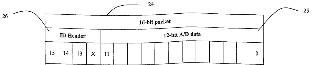
Figure 5a: Transmission Data Format
