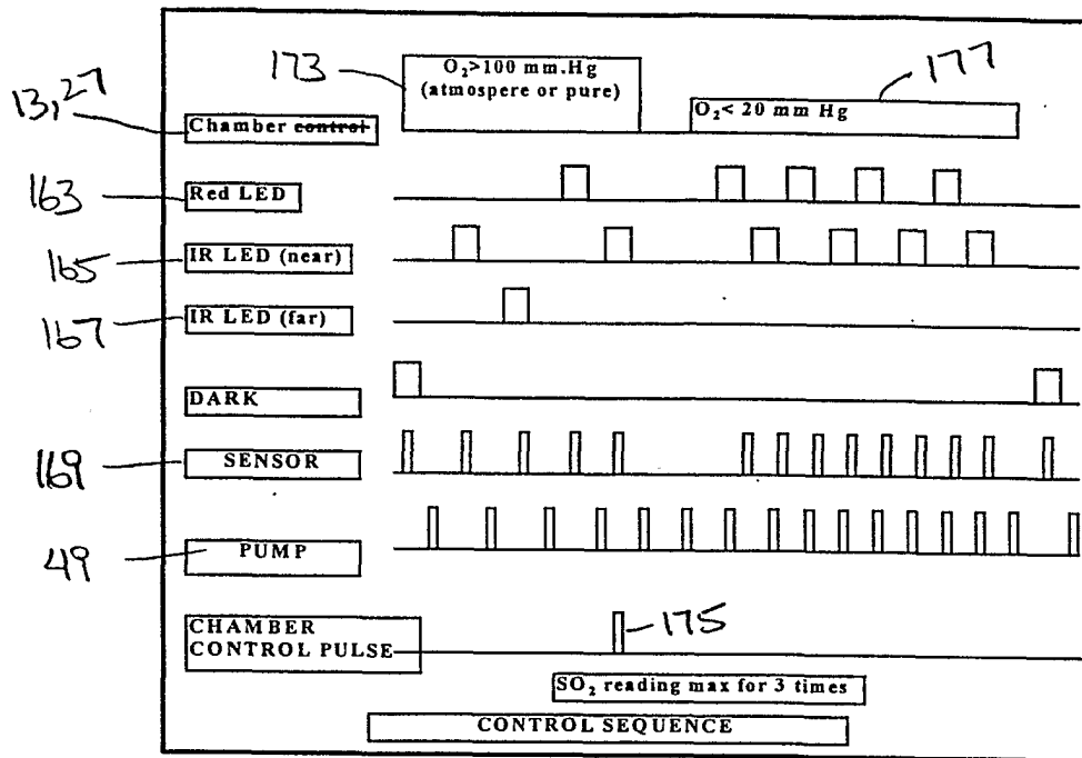
Figure : Sensor, pump and environmental control sequence
